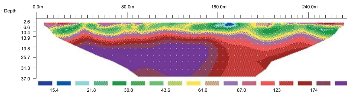
Inverse Model Resistivity Section (Ohm x m)
