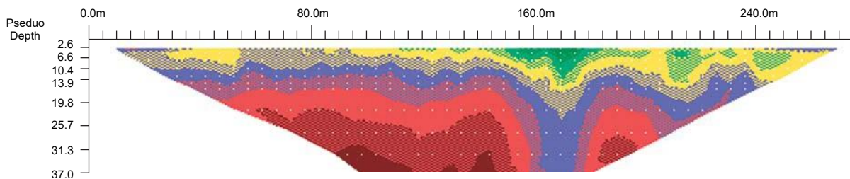
Measured Apparent Resistivity Pseudosection
