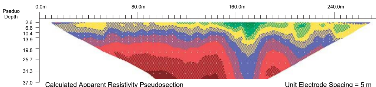
Calculated Apparent Resistivity Pseudosection
