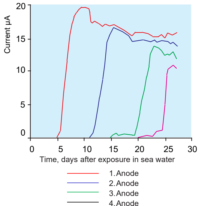
Figure 1. Increase in current in the 4 anodes
