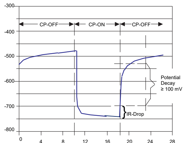
Figure 1: Polarisation Curve from CP-System
